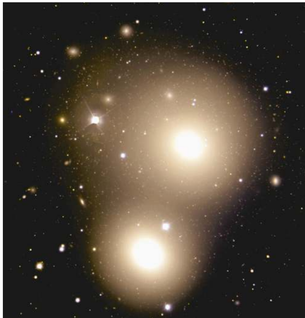
Two elliptical galaxies: NGC 3311 and NGC 3309.
